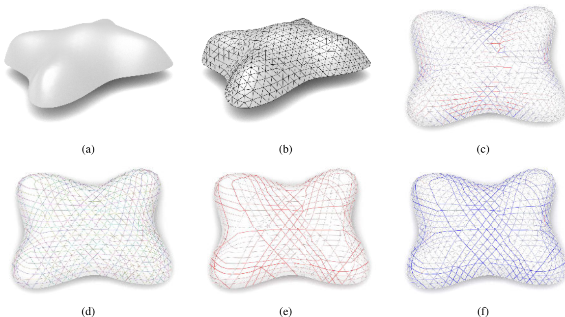
Figure 4: Our processing pipeline shown for the Simplilium case study of Figure 1: (a) the input mesh; (b) the regular remeshing computed using [JTSPH15]; (c) the stress on the linear truss model subject to an external load (blue is compression, red is tension); (d) the candidate cables; (e) the chosen cables and their pre-load; (f) the final stress.
