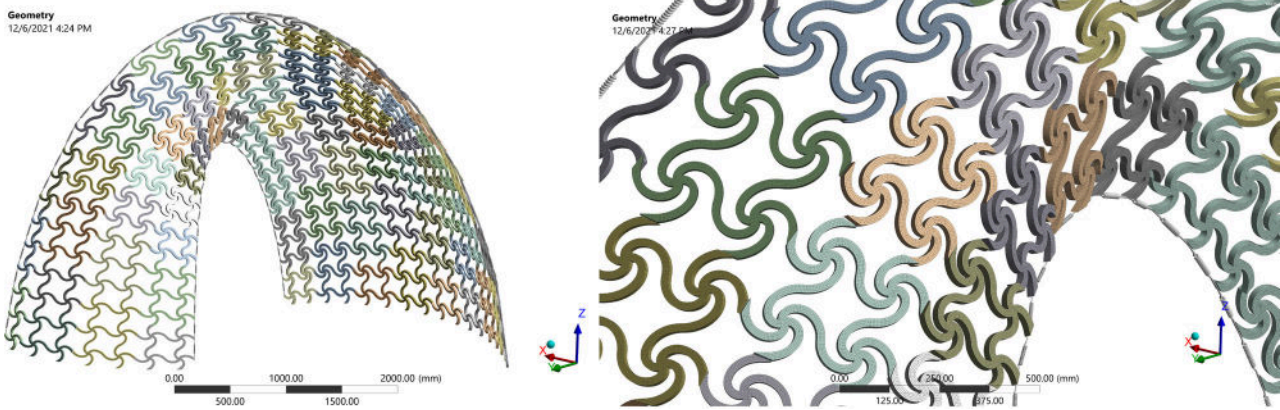
Figure 8: FE model of the structure at the starting point before pre-stress (i.e. where the panels are not in contact but are floating in the flat configuration). The springs, the boundary conditions and the internal restraints are birth/death elements)
