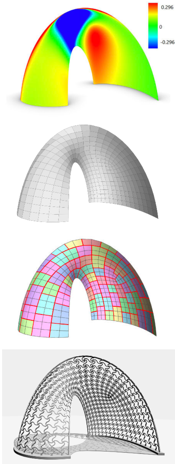
Figure 6: Computational design, from top to bottom: Gaussian curvature, quad mesh, patches, final design
