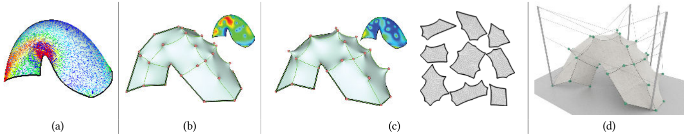
Fig. 2. Processing pipeline overview: (a) Starting from a triangle mesh equipped with a smooth curvature-aligned cross field; (b) we compute an optimal patch layout that accounts for the physical simulation of the resulting tensile structure; (c) we refine the anchor point positions through a final optimization step to minimize the deviation from the target surface and enhance developability, the approximation error is visualized, with red indicating 5% of the bounding box diagonal; (d) optionally, we compute an optimized cable configuration to ensure structural equilibrium.
