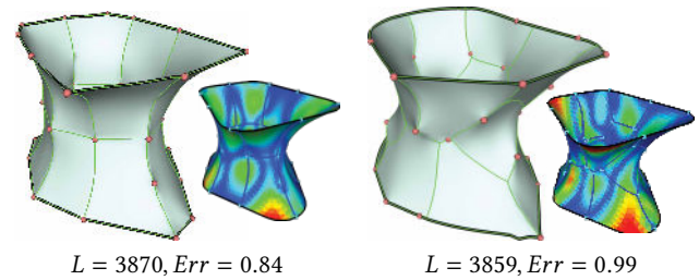
Fig. 9. Comparison between different partitioning strategies used to derive the tensile structure: our field-based optimization (left) versus a Voronoi-based partitioning (right), both processed using our membrane derivation method. Each experiment reports the total seam length and the average Hausdorff distance from the target surface.
