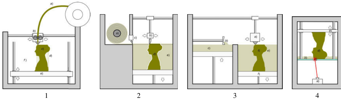
Figure 2: The four main additive fabrication technologies described in section 2.2; from left: Fused Deposition Modelling, Laminated Object Manufacturing, Granular Binding, and Photopolymerization
