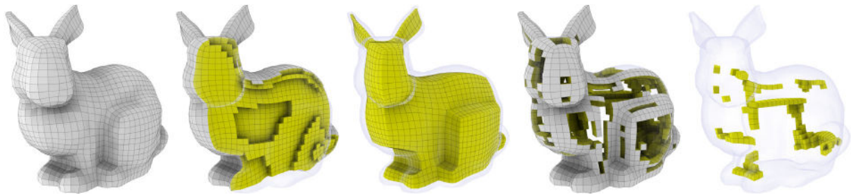
Fig. 2. Examples of HexaLab filters applied to a hex-mesh to reveal its interior. From left to right: complete, unfiltered model; slicing-plane filter; peeling filter (two most external layers of cells removed); quality-thresholding filter (hexas with SJ < 0.96 are shown); and the combination of all these filters. Source: “Bunny” model courtesy of [2].
