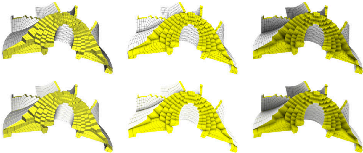
Fig. 5. The lighting modes offered by HexaLab. From left to right: direct illumination only, global illumination approximated with Screen Space Ambient Occlusion (SSAO), and with Object Space Ambient Occlusion (OSAO), which is HexaLab default. Global illumination schemas are more demanding, but are more effective at conveying the 3D space, especially OSAO. Bottom: the improvement is further enhanced when “rounded modes” are used to separate elements. Source: Model courtesy of [1].
