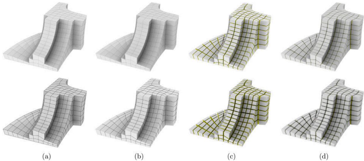
Fig. 3. (a) the traditional rendering of \mathcal{M}_S to represent \mathcal{M}_V . (b) darkness-coded mode. (c) crack mode. (d) rounded mode. Bottom row: the same modes, for a different selection of darkness/width/radius. Source: Model courtesy of [1].
