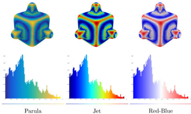
Fig. 10. Different color mappings on hex quality (top), and associated histograms (bottom).
