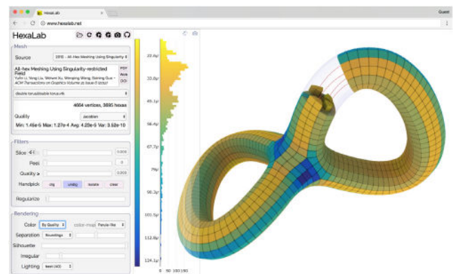
Fig. 1. A screen-shot of HexaLab running inside Chrome under macOS. Source: Model courtesy of [1].
