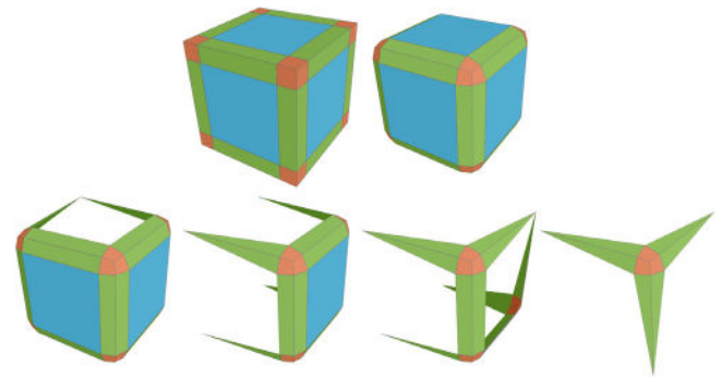
Fig. 13. Boundary polygons produced for a hexacell (to be rendered and lit). Top: topological subdivision and geometrical displacement. Bottom: examples of the produced polygons for four different configurations of six, four, three, and one “exposed” vertices. (For interpretation of the references to color in this figure legend, the reader is referred to the web version of this article.)
