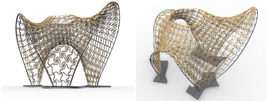
Fig. 21. Shape comparison between the theoretical deformed shape (colored) as outcome of the FE analysis and the real scan data (gray).
