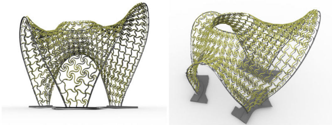
Fig. 22. Shape comparison between the theoretical deformed shape (colored) as outcome of the FE analysis and the real scan data (gray). The FE model has been updated considering the new position of the ground faces, as surveyed through the scan session.
