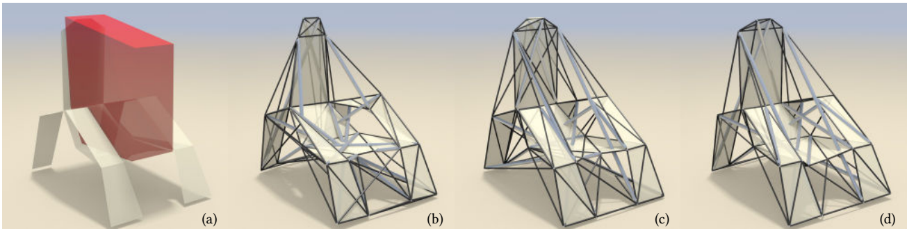
Fig. 12. Three variations on a “tensegrity chair”, obtained from the same input mesh (on the left) and collision mesh (in red) to keep the seating area free. The variations are obtained for various choices of connectivity-finding parameters: normal orientation, random, and maximal total length (Section 5.1).
