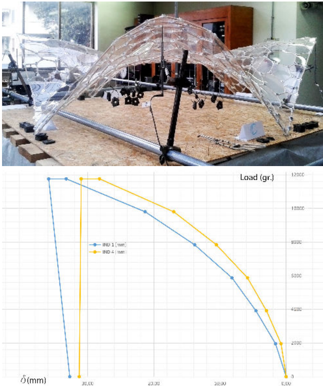
Figure 10: (a) The load test performed on the fabricated mockup; (b) The load/displacement ratio.
