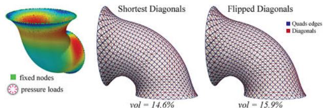
Fig. 18. Effects of the choice of diagonal directions: on the left, the original diagonals computed by our method, choosing the shorter diagonal; on the right, the diagonals of the first boundary ring are preserved and internal ones are flipped.
