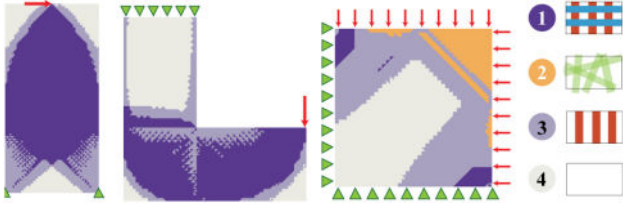
Fig. 13. Zones of an optimal strain field. (1) Two orthogonal directions, (2) no preferred direction, (3) one direction, (4) no beams. The crossfield directions are well-defined only for regions 1 and 3.
