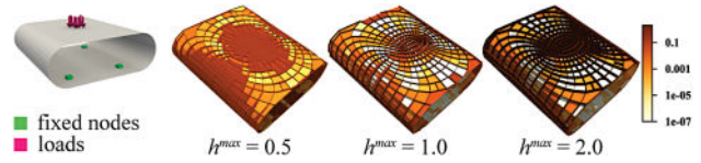
Fig. 22. In a bending dominated structure, changing the maximal allowed thickness from small to large causes the results to change from a solid plate to a rib-like structure.
