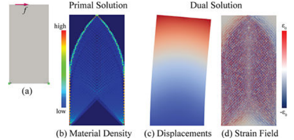
Fig. 10. Field optimization: (a) Design domain \Omega and boundary conditions; (b) Primal solution, squared densities \sqrt{\rho_1 + \rho_2} ; (c,d) Dual solutions, displacements \mathbf{u} and strain \varepsilon eigen-values and -vectors.
