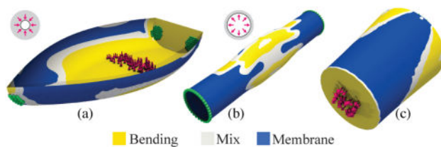
Fig. 5. Loaded shells dominated by bending and membrane forces and a mix of these. Support nodes are highlighted in green while loads are shown in red. Loads on (a) and (b) include, respectively, external and internal pressure.
