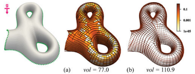
Fig. 24. Optimization results using different volume formula: (a) exact volume and (b) approximate convex volume.
