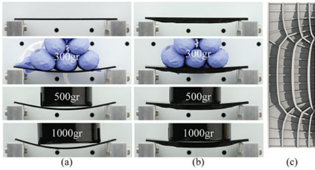
Fig. 26. (a) Shelf of uniform thickness; (b) optimized shelf of same weight; (c) model of optimized shelf.
