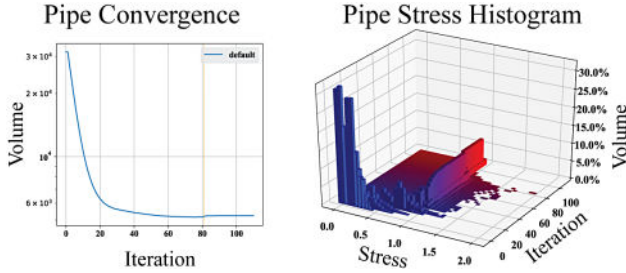
Fig. 20. Convergence plots for the Pipe model (Figure 29(d)). On the left, the volume vs. iteration count; On the right, the evolution of the histogram of the stress where volume percentage is measured with respect to the initial volume. At iteration 81, we start the post-process that ensure stresses are below \sigma_0 = 1 .
