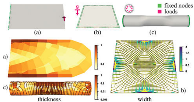
Fig. 3. (a) Optimal structure for a standard cantilever test case with variable thickness [Sigmund et al. 2016]; (b) bending plate optimization, subject to uniform vertical loads, resulting in a rib structure qualitatively consistent with analytic results; (c) an optimized pipe structure, subject to internal pressure, exhibiting a mix of behaviors.
