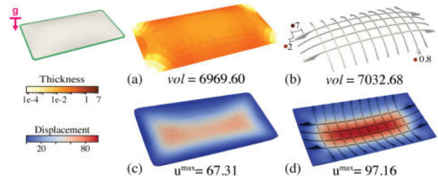
Fig. 25. Finite Element Analysis of reinforced structures: (a) variable thickness reinforcement generated by our system; (b) rib-reinforcement from Li et al. [2017]; (c–d) simulated displacements on reinforced structures.
