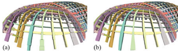
Fig. 14. Inflation: (a) Each block is meshed independently, leading to a visible artifact; (b) An entire stream of edges is meshed to produce a smoother result.
