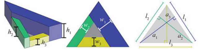
Fig. 7. Geometric parametrization of triangular cell. Left: perspective view of the three blocks; Center: top view showing widths; Right: triangle sides l_i and respective triangle heights a_i .
