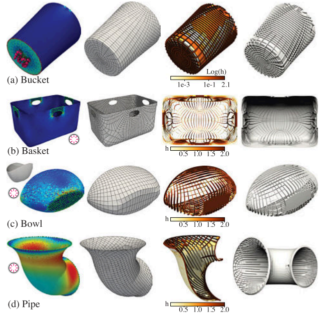
Fig. 29. Examples of consumer product objects. For each one, images show loads and initial stress distribution, quad-rangulation, cell optimization colored by thickness, and final geometry.
