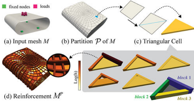
Fig. 6. Perforated variable thickness shell. (a) Input triangle mesh M with boundary conditions; (b) partition \mathcal{P} of the input into polygonal faces; (c) each triangular subcell comprises three trapezoidal blocks; (d) extruded cells forming variable-thickness shell structure M^P .
