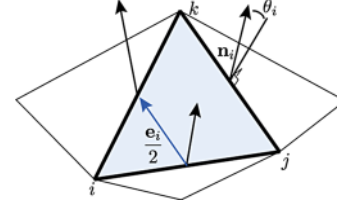
Fig. 12. Discretization of the bending field.
