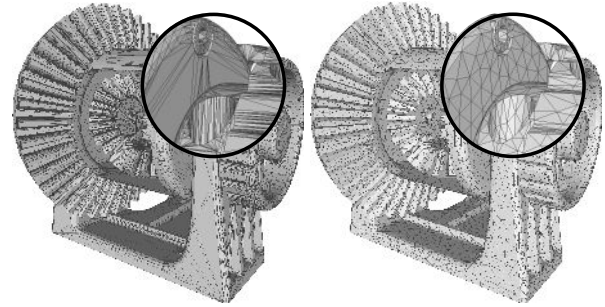
Fig. 4. The effect of adaptive remeshing on one mechanical object from the Thingi10k [Zhou and Jacobson 2016] repository.
