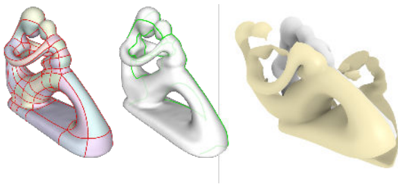
Figure 12: FlexMolds [MPBC16] presents an automatic method for the generation of flexible molds defined as a thin layer of elastic material. The method automatically optimizes the cut layout required to open the mold and release the cast, based on a physically-based simulation of the extraction process.
